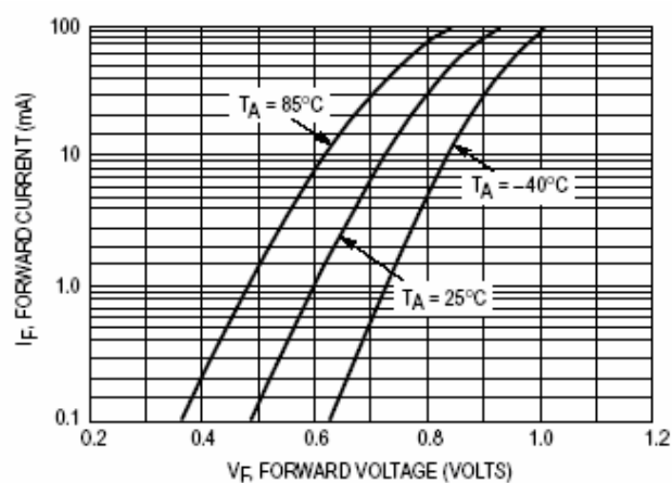
Figure 1. Forward Voltage
