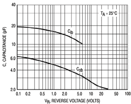
Figure 11. Capacitance
