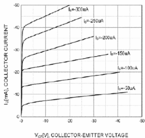
Static Characteristic
