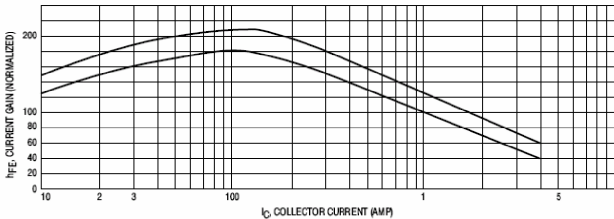
Figure 2. Current Gain
