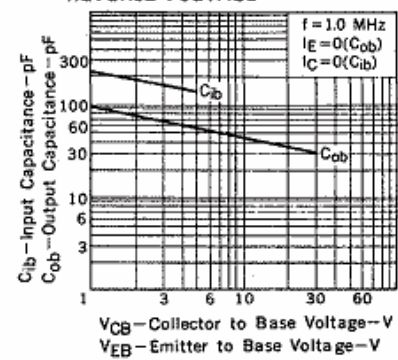
INPUT AND OUTPUT CAPACITANCE vs. REVERSE VOLTAGE
