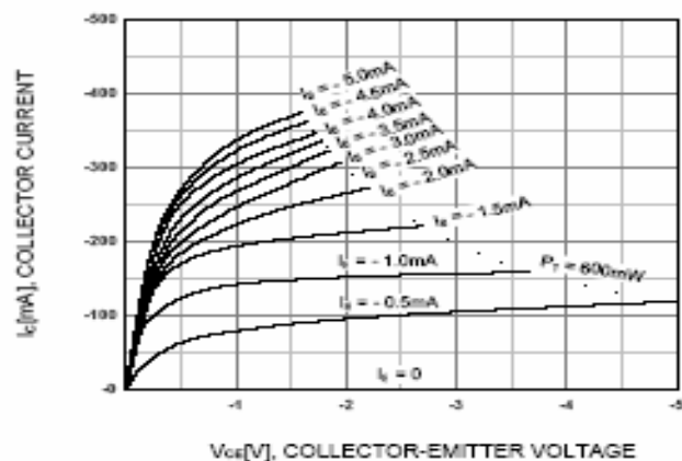
Figure 1. Static Characteristic
