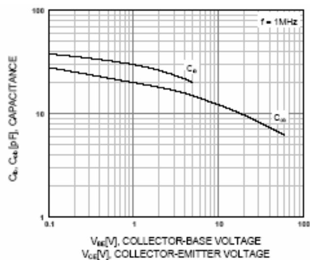
Figure 7. Input and Output Capacitance vs. Reverse Voltage
