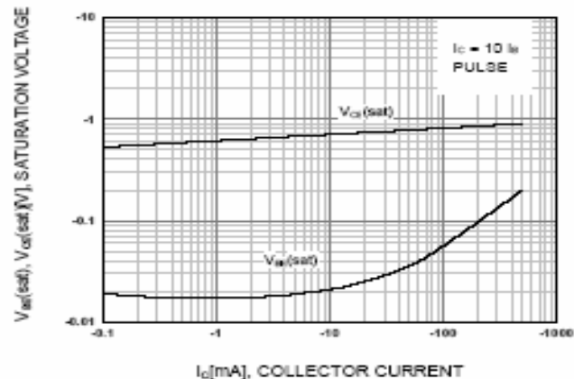
Figure 4. Base-Emitter Saturation Voltage Collector-Emitter Saturation Voltage
