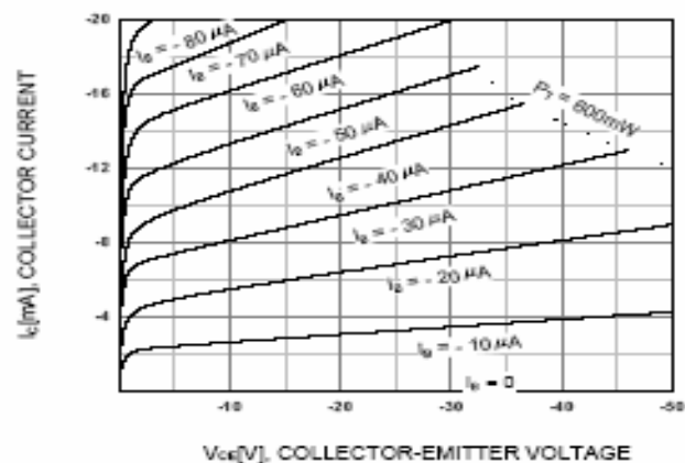
Figure 2. Static Characteristic
